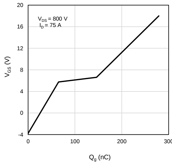
Figure 12: Gate-Charge Characteristics
